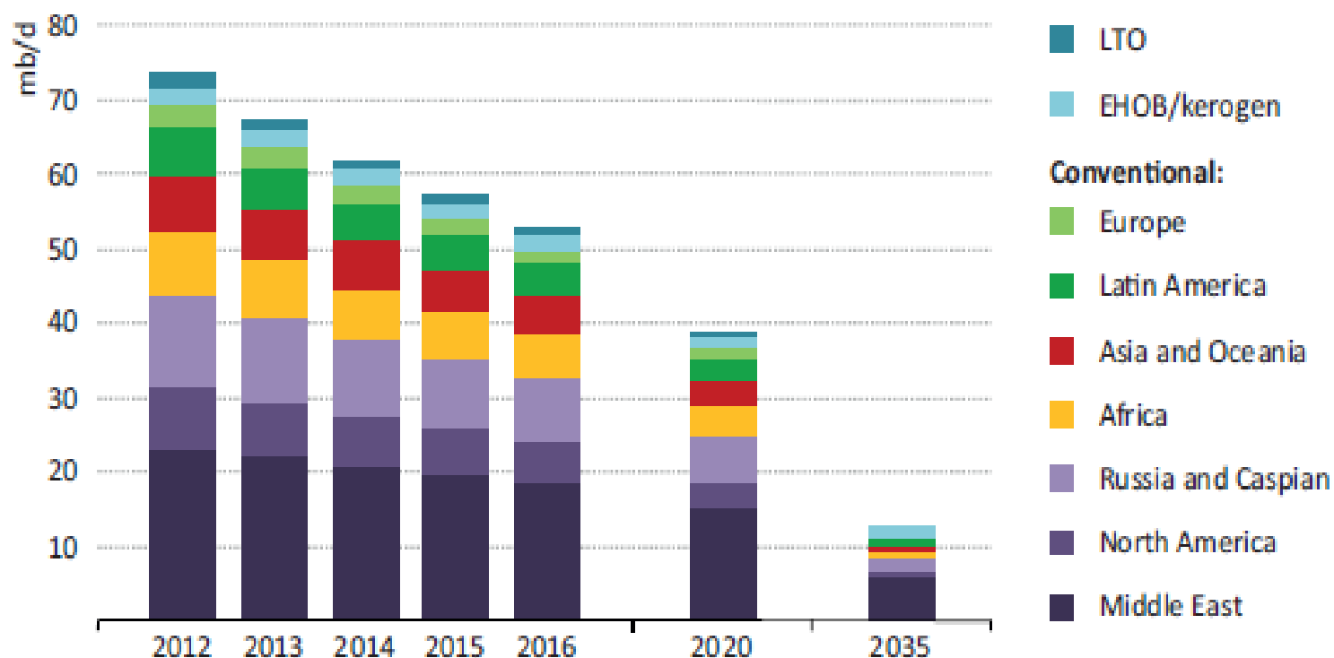
Figure 14.6 ▶ Production that would be observed from all currently producing fields in the absence of further investment (excluding NGLs)
